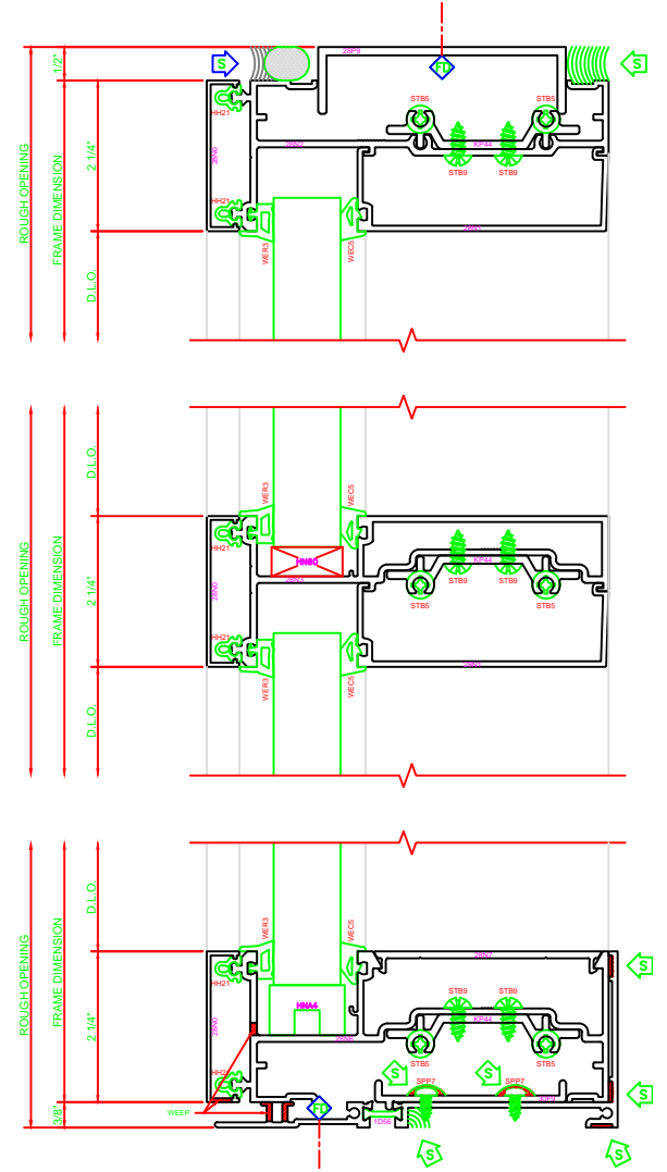
101 HEAD SERIES: 600R
