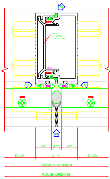
605 SSG EXP. VERT. SERIES: 600R
