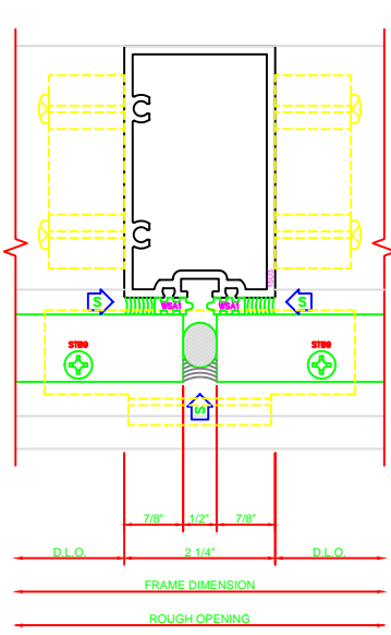
604 SSG VERTICAL SERIES: 600R
